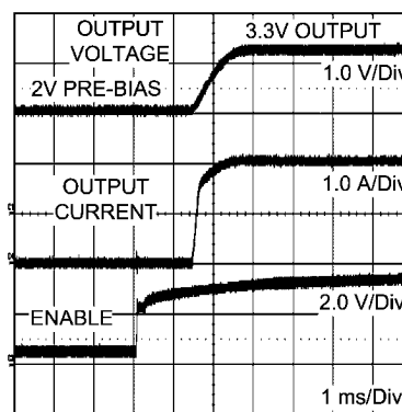
Pre-Biased Startup
