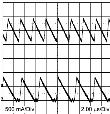
CCM and DCM Operating Modes V_{IN} = 24V , V_O = 3.3V , I_O = 2A/0.32A 2 \mu\text{sec/div}
