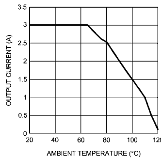
Thermal derating curve V_{IN} = 24\text{V} , V_{OUT} = 5.0\text{V} ,
