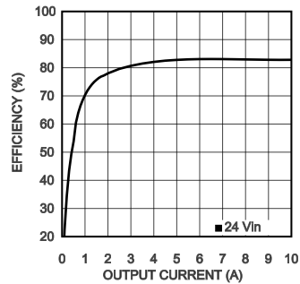
Efficiency V_{IN} = 24\text{V} V_{OUT} = 3.3\text{V}
