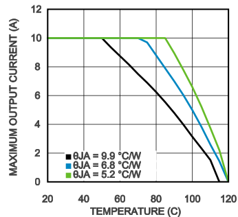
Thermal derating curve V_{IN} = 24\text{V} , V_{OUT} = 3.3\text{V}
