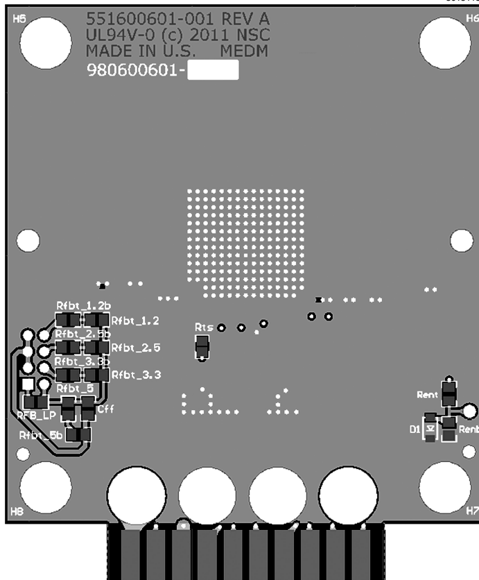
FIGURE 6. Layout example
