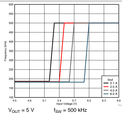
Figure 42. Frequency Foldback
