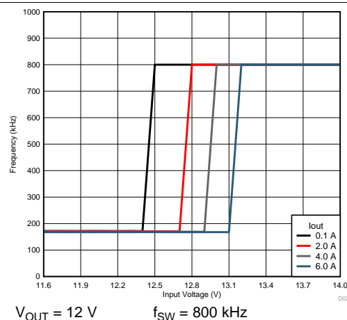
Figure 44. Frequency Foldback
