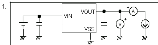
Circuit 1
