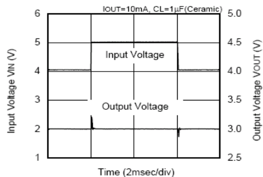
Input Transient Response
