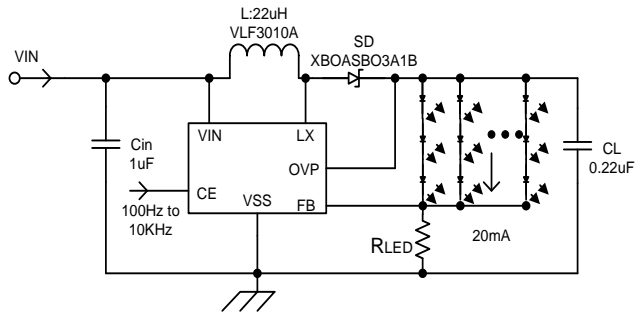
Circuit 3
