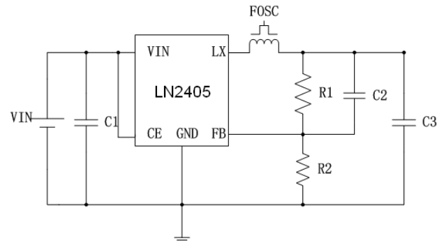
Circuit 2
