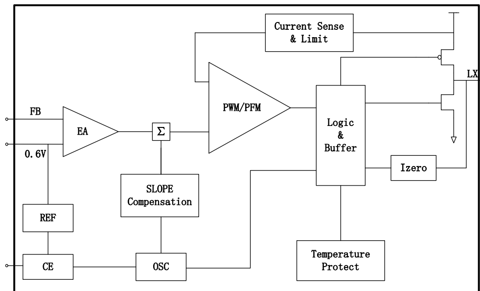
LN5070 half functional block diagram (symmetric structure)
