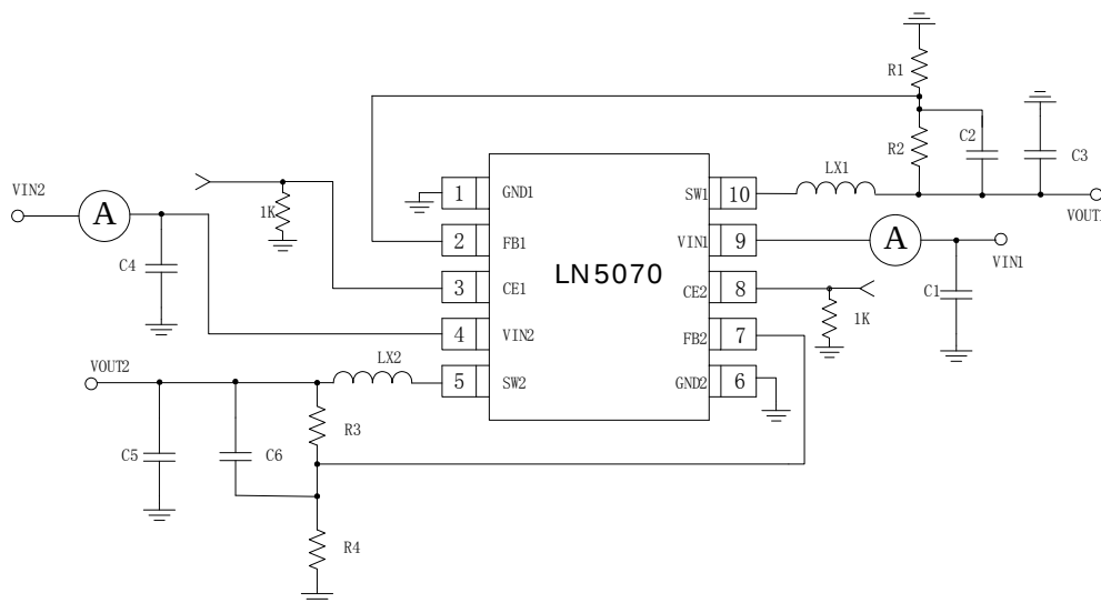
Circuit 1
