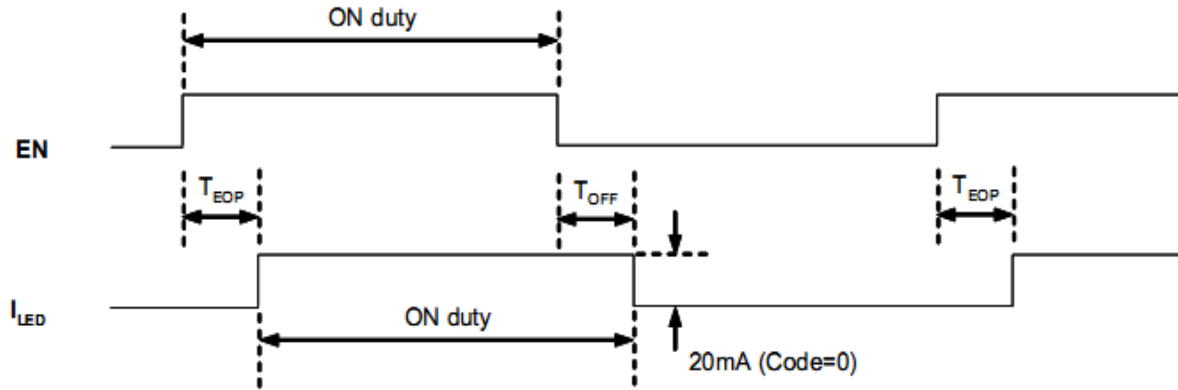
Fig1. Turn On To PWM Dimming
