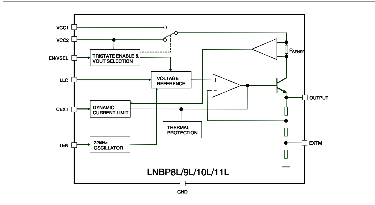
Figure 1. Block diagram
