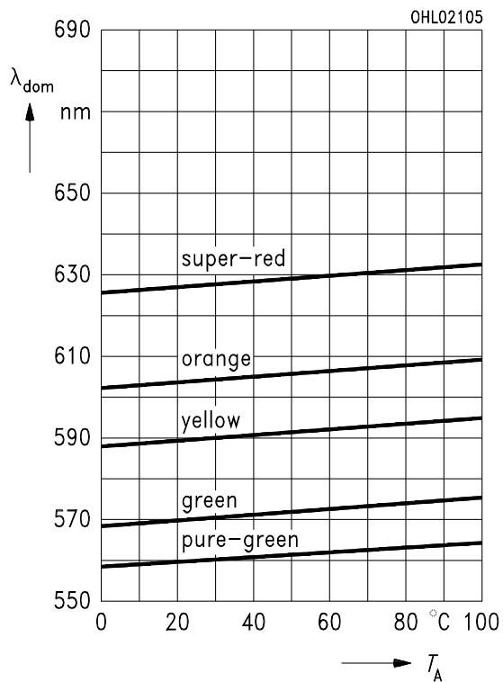
Dominantwellenlänge \lambda_{dom} = f(T_A) Dominant wavelength I_F = 20 mA
