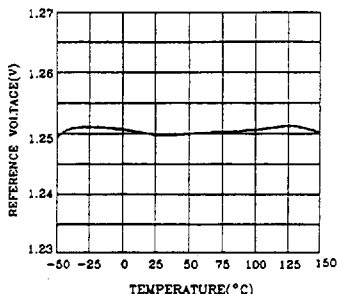
Temperature Stability
