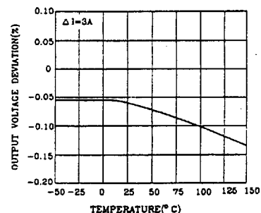
LT1085 Load Regulation
