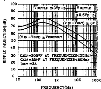
LT1085 Ripple Rejection
