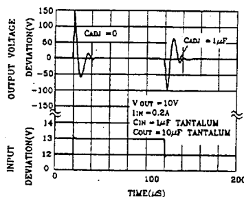
LM1084 Line Transient Response
