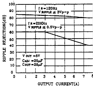
LT1083 Ripple Rejection vs Current
