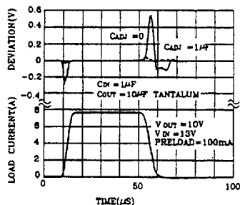
LM1083 Load Transient Response
