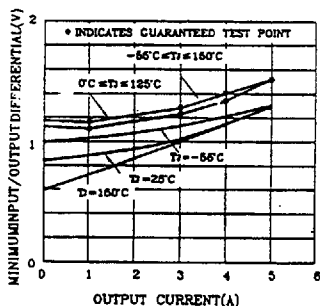
LT1084 Dropout Voltage
