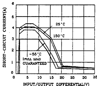
LT1085 Short-Circuit Current
