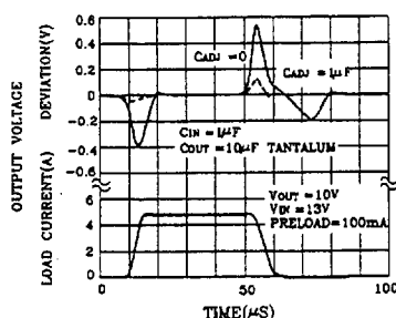
LM1083 Load Transient Response
