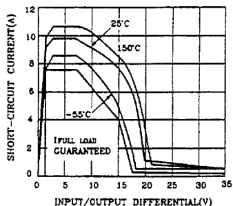
LT1083 Short-Circuit Current
