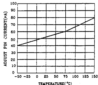
Adjust Pin Current
