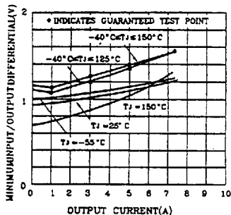
LT1083 Dropout Voltage
