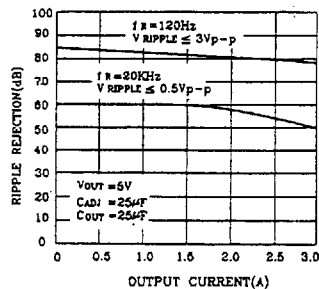
LT1084 Ripple Rejection vs Current
