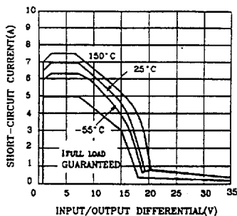
LT1084 Short-Circuit Current
