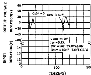
LM1085 Line Transient Response
