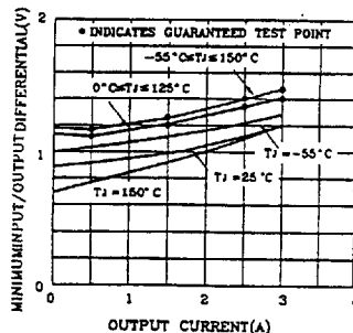
LT1085 Dropout Voltage
