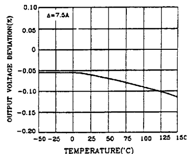
LT1083 Load Regulation
