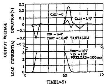
LM1083 Load Transient Response
