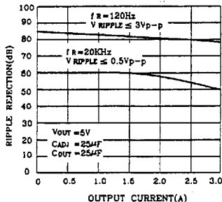
LT1085 Ripple Rejection vs Current
