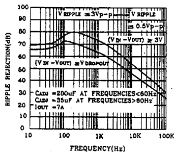
LT1083 Ripple Rejection
