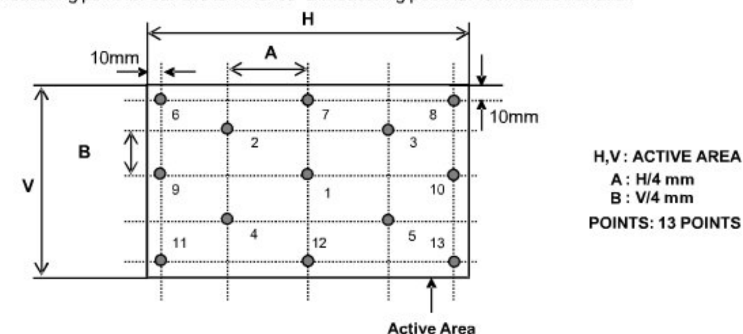
FIG. 3 Response Time
