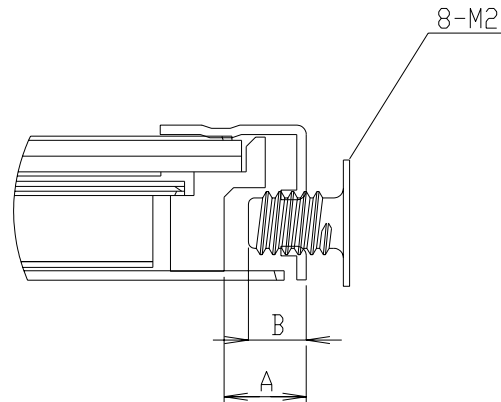
SECTION A-A SCALE 5/1
