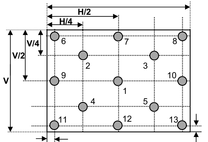
Luminance variation measurement 13 points
