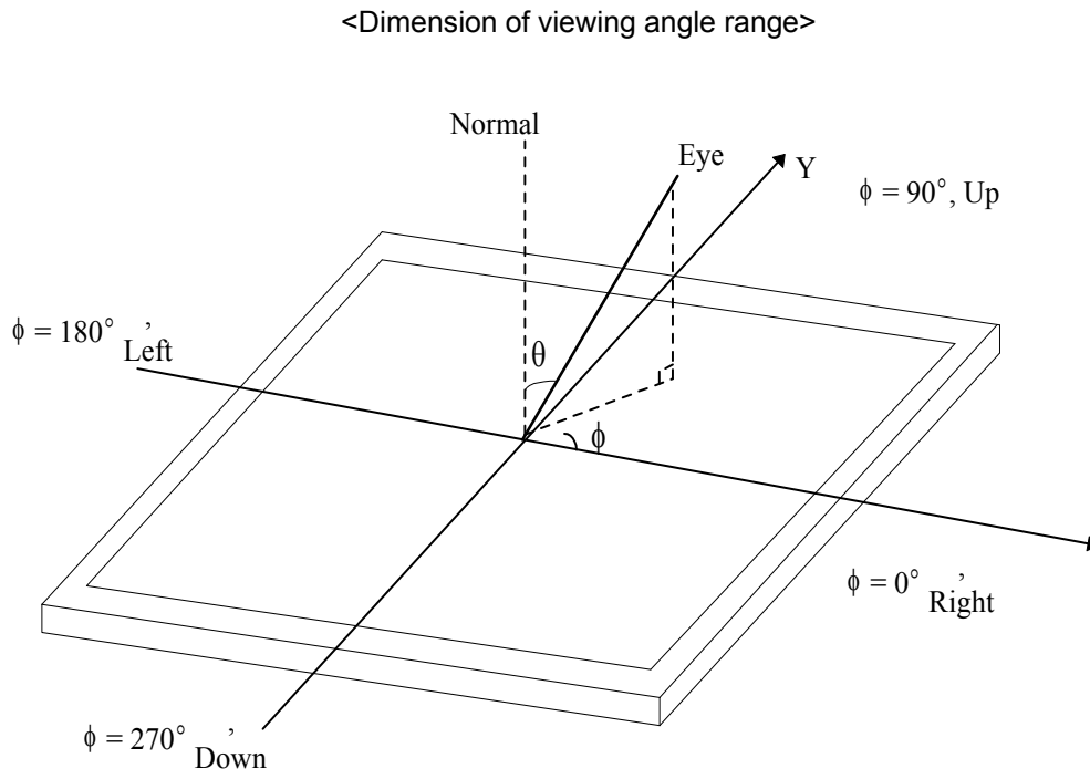
FIG. 4 Viewing angle
