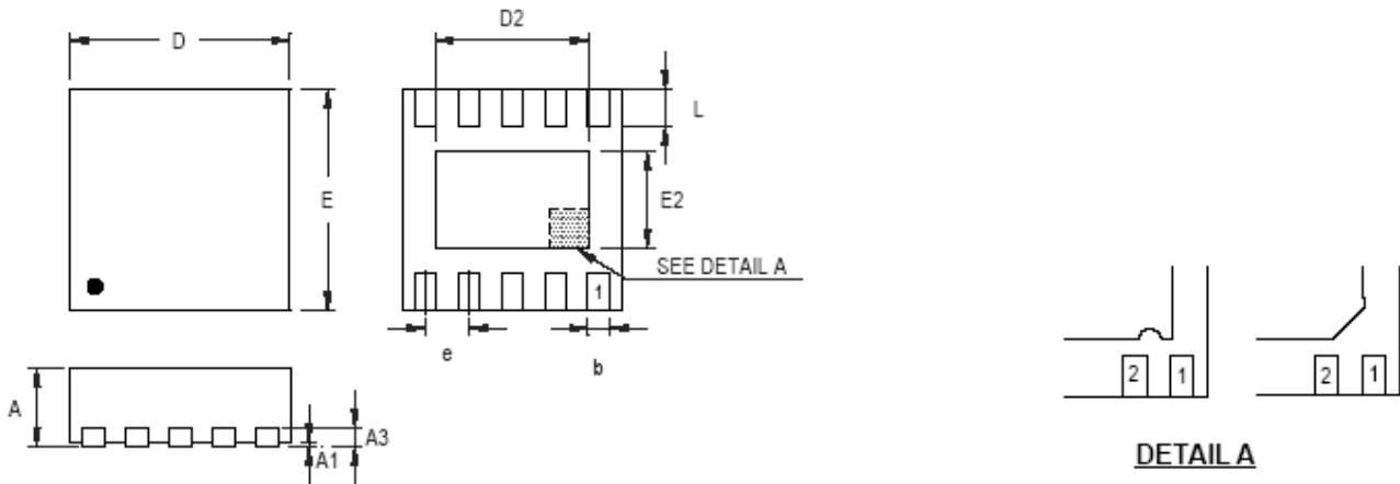
Pin #1 ID and Tie Bar Mark Options
