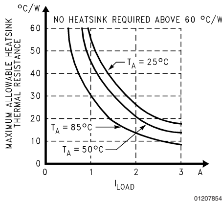
FIGURE 8. Heatsink Thermal Resistance Requirements for Figure 7
