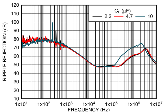
Figure 5-21. Ripple Rejection vs Output Capacitor ( C_L ) and Frequency (New Chip)
