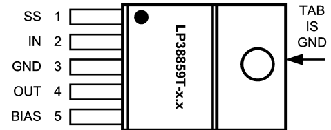
TO220-5, Top View
