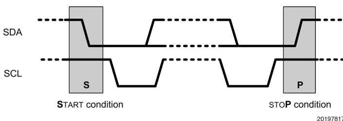
START and STOP Conditions
