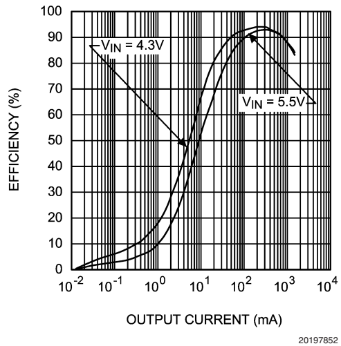
Buck 2 Efficiency vs Output Current (Forced PWM Mode, V_{out} = 3.3\text{V} , L = 2.2\mu\text{H} )
