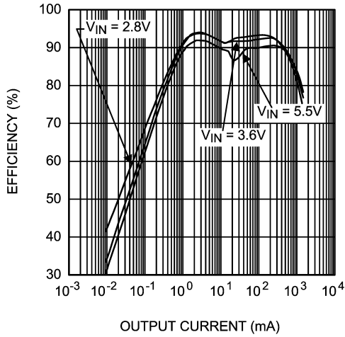
Buck 1 Efficiency vs Output Current (PFM to PWM mode, V_{out} = 1.2\text{V} , L = 2.2\mu\text{H} )
