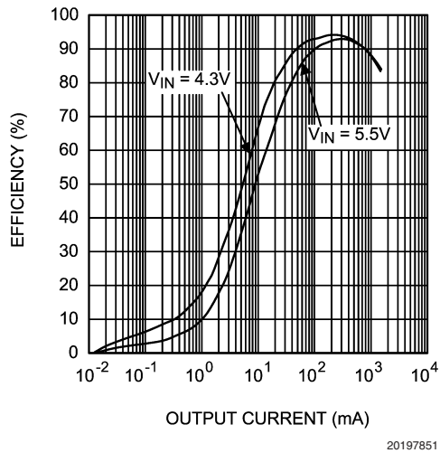
Buck 2 Efficiency vs Output Current (Forced PWM Mode, V_{out} = 1.8\text{V} , L = 2.2\mu\text{H} )
