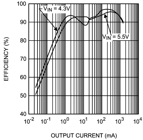
Buck 2 Efficiency vs Output Current (PFM to PWM Mode, V_{out} = 3.3\text{V} , L = 2.2\mu\text{H} )
