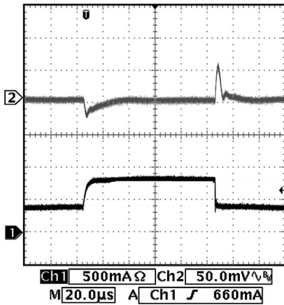
Load Transient Response V_{out} = 1.2 (PWM Mode)
