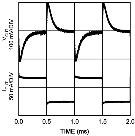
Boost Load Transient Response 25mA – 70mA
