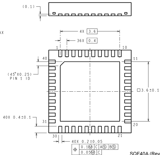
40-Pin LLP NS Drawing SQF40A
