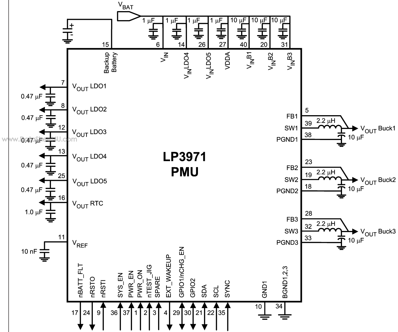
Diagram 1 LDO 4 and LDO5 Connected To V BATTERY
