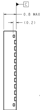
40-Pin LLP NS Drawing SQF40A
