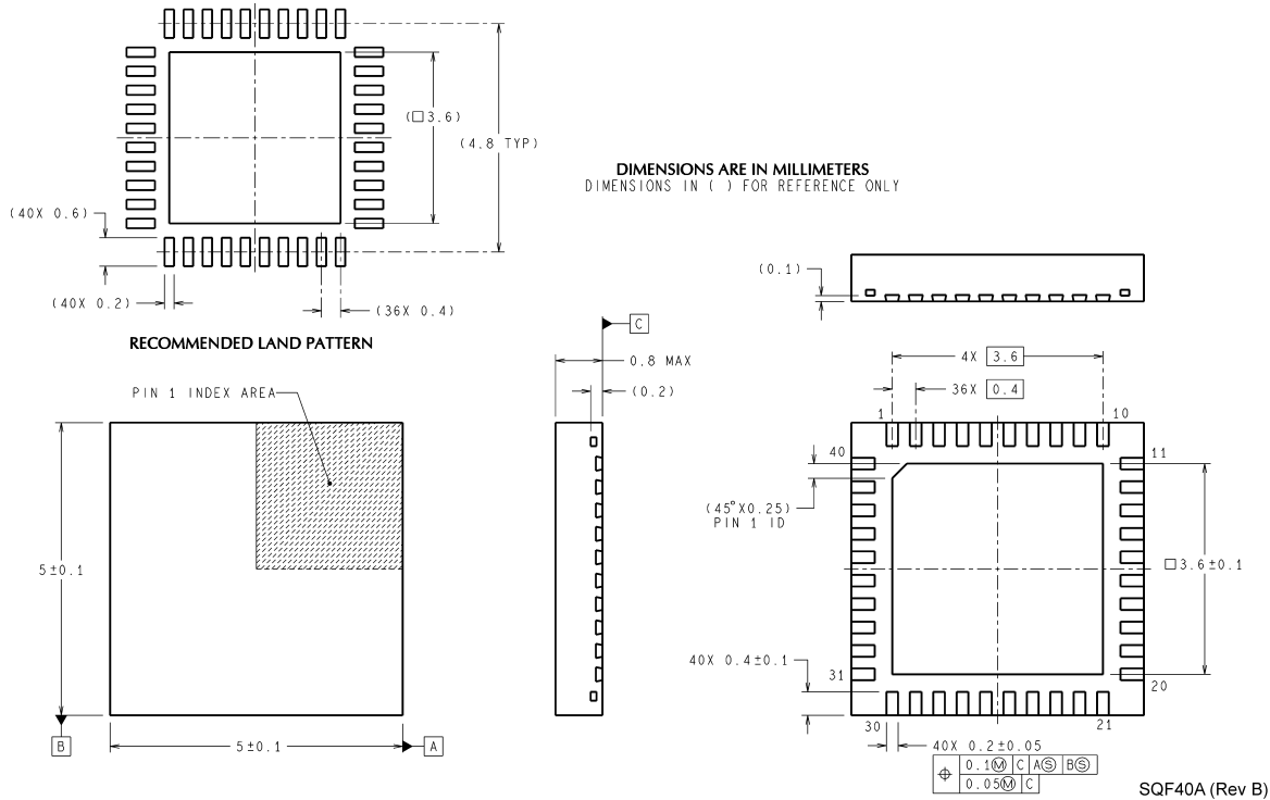
40-Pin Leadless Leadframe Package NS Package Number SQF40A
