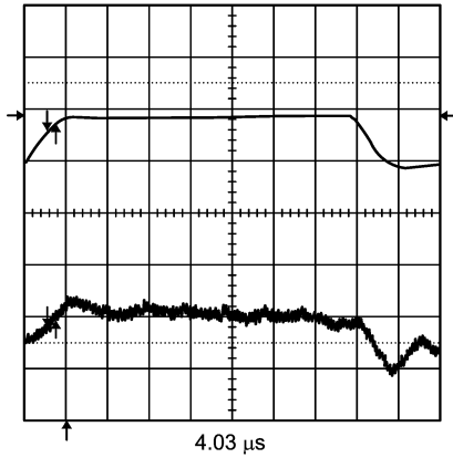
Load Transient 3.6 V IN , 3.3 V OUT , 0 – 100 mA load
