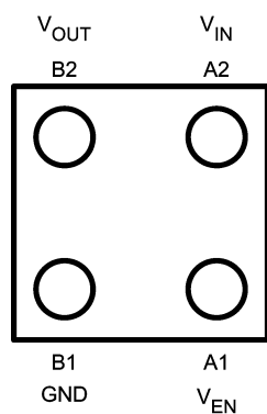
Bottom View
