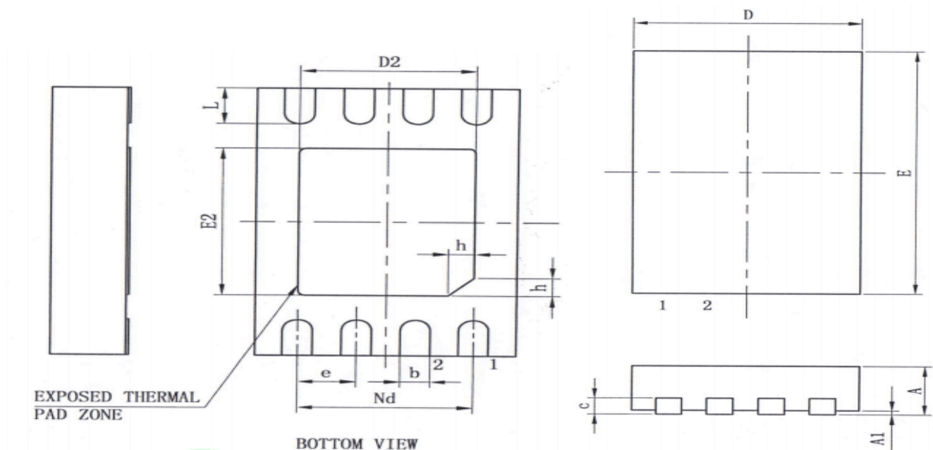
DFN-8
