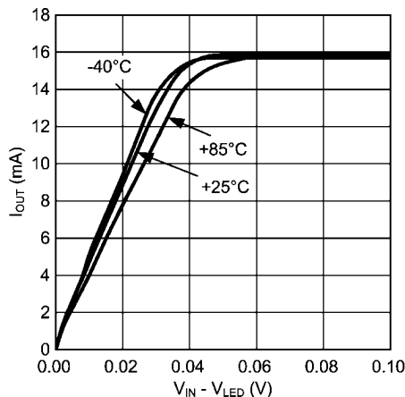
Output Current vs Headroom Voltage
