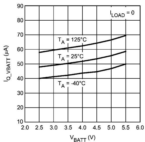
Quiescent Current I Q_VBATT vs V BATT
