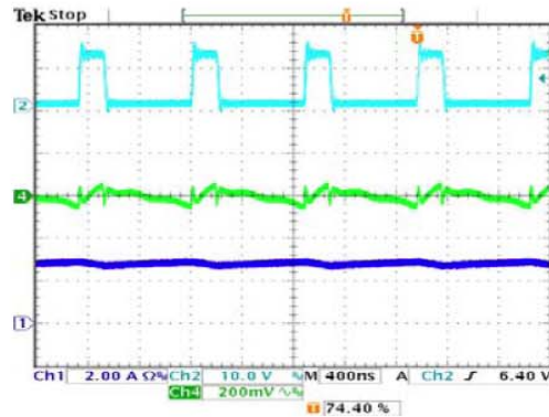
CH1=Inductor Current,CH3=LX,CH4= V_{OUT} AC-Coupled V_{CC}=3.3V , V_{OUT}=12V I_{LOAD}=600mA Freq=1.2MHz
