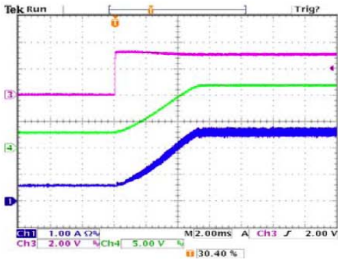
CH1=Inductor Current,CH3=EN,CH4= V_{OUT} V_{CC}=3.3V , V_{OUT}=12V I_{LOAD}=600mA Freq=640KHz
