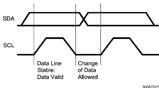
FIGURE 1. Bit Transfer
