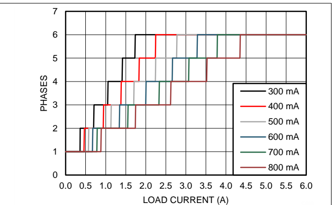
Figure 3. Phase Shedding vs Load Current with Different Level Settings
