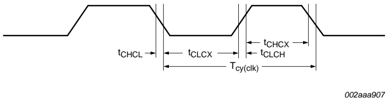
Fig 24. External clock timing (with an amplitude of at least V_{i(RMS)} = 200\text{ mV} )
