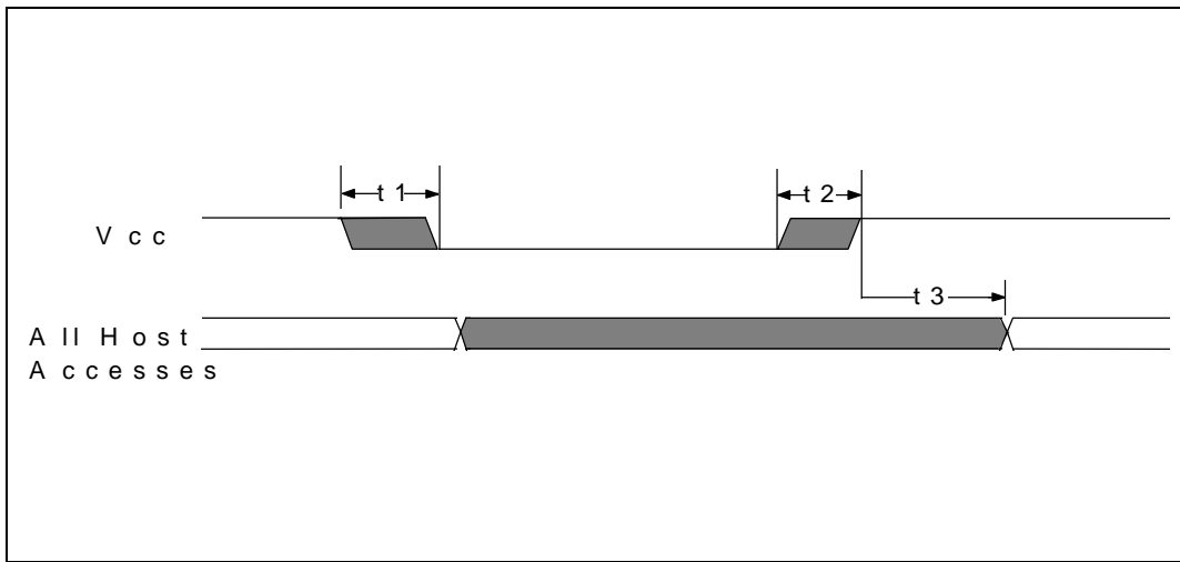
FIGURE 15 - POWER-UP TIMING
