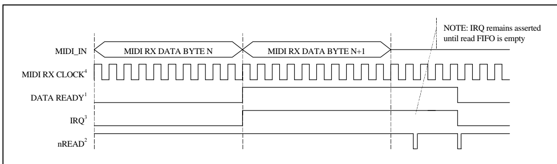
FIGURE 4 - MPU-401 INTERRUPT
