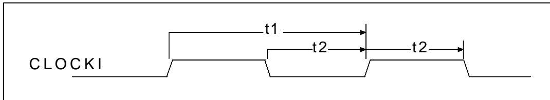
FIGURE 16A - INPUT CLOCK TIMING
