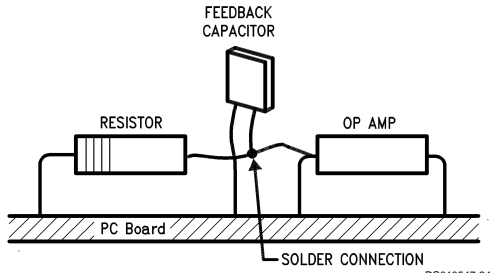
FIGURE 6. Air Wiring
