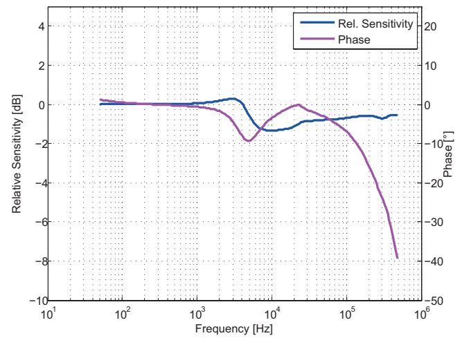
Figure 7: Frequency response
