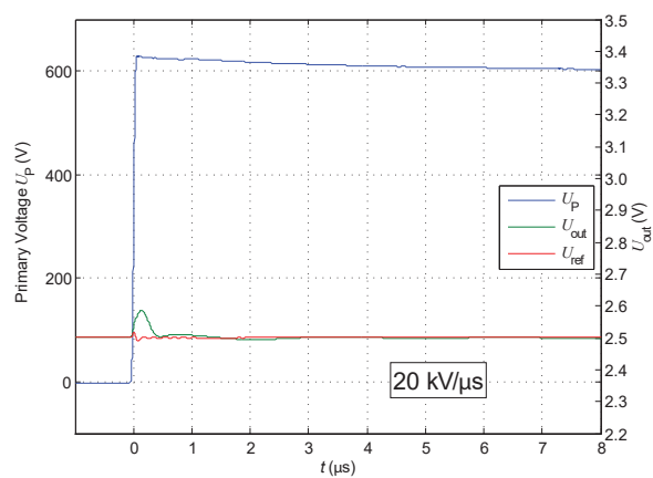
Figure 15: du/dt
