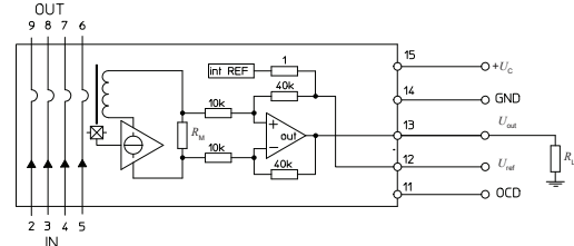
Figure 26: Test connection
