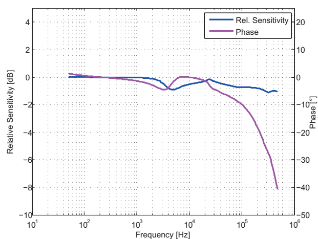
Figure 2: Frequency response
