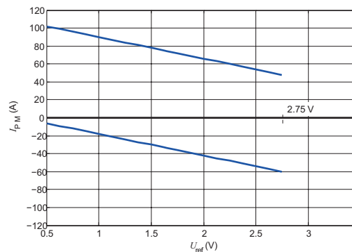
Figure 31: Measuring range versus external U_{ref} LPSR 15 A
