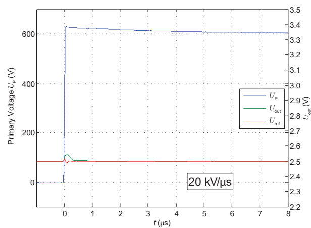
Figure 20: du/dt
