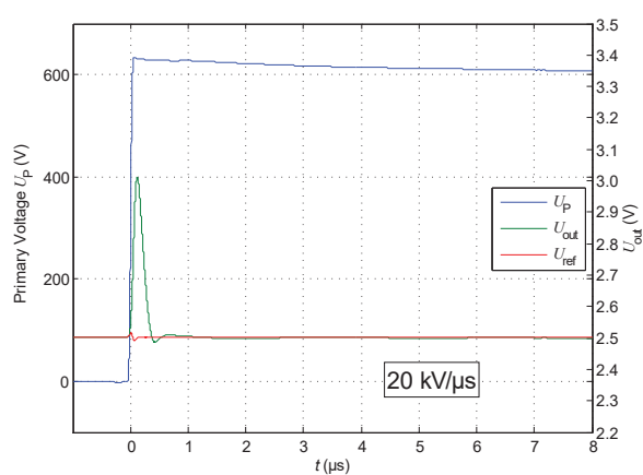
Figure 5: du/dt
