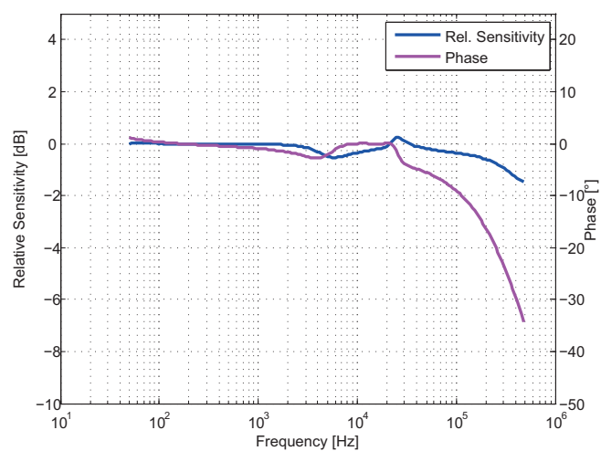
Figure 17: Frequency response
