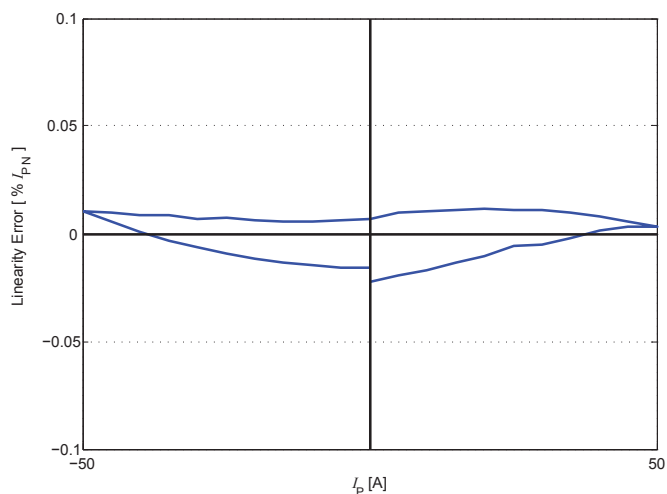
Figure 16: Linearity error
