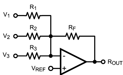
FIGURE 3. Summing Amplifier Circuit
