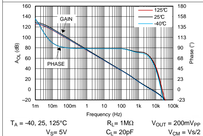
Figure 35. Open Loop Gain and Phase, 5V, 1 MΩ Load
