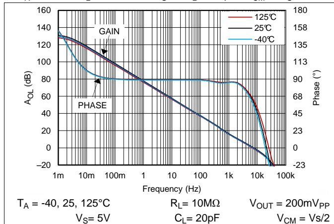
Figure 33. Open Loop Gain and Phase, 5V, 10 MΩ Load
