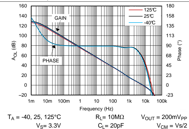
Figure 34. Open Loop Gain and Phase, 3.3V, 10 MΩ Load
