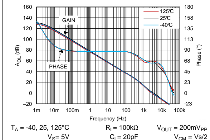
Figure 37. Open Loop Gain and Phase, 5V, 100kΩ Load
