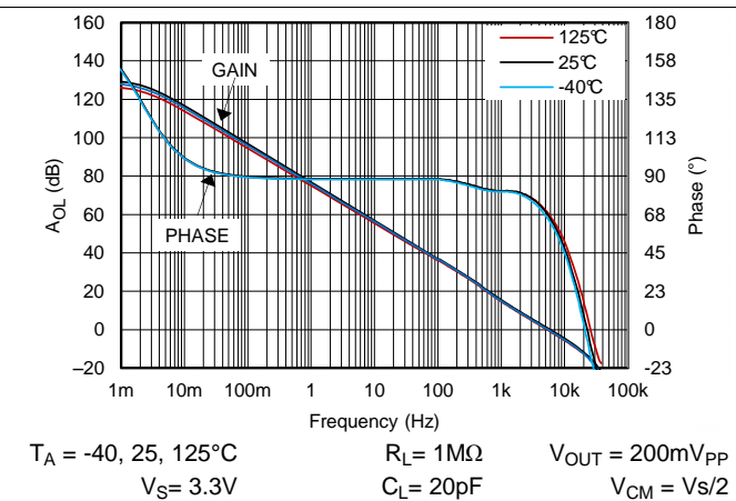
Figure 36. Open Loop Gain and Phase, 3.3V, 1 MΩ Load
