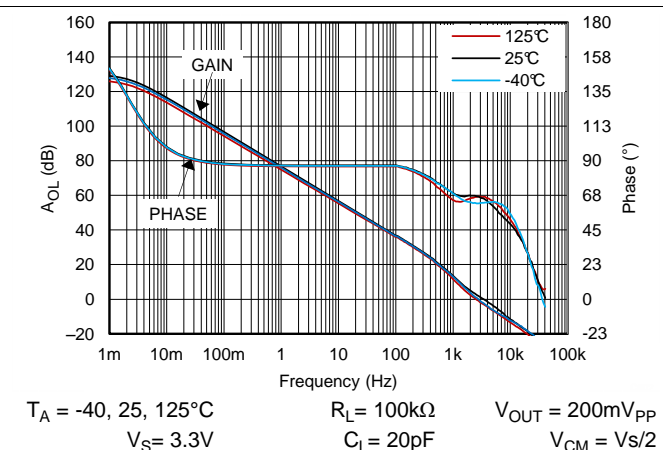
Figure 38. Open Loop Gain and Phase, 3.3V, 100kΩ Load
