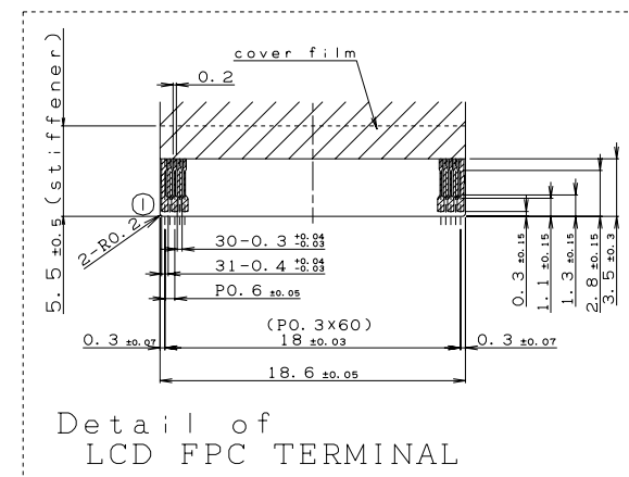
Fitting CN:Hirose FH23-61S-0.3SHAW(O5)
