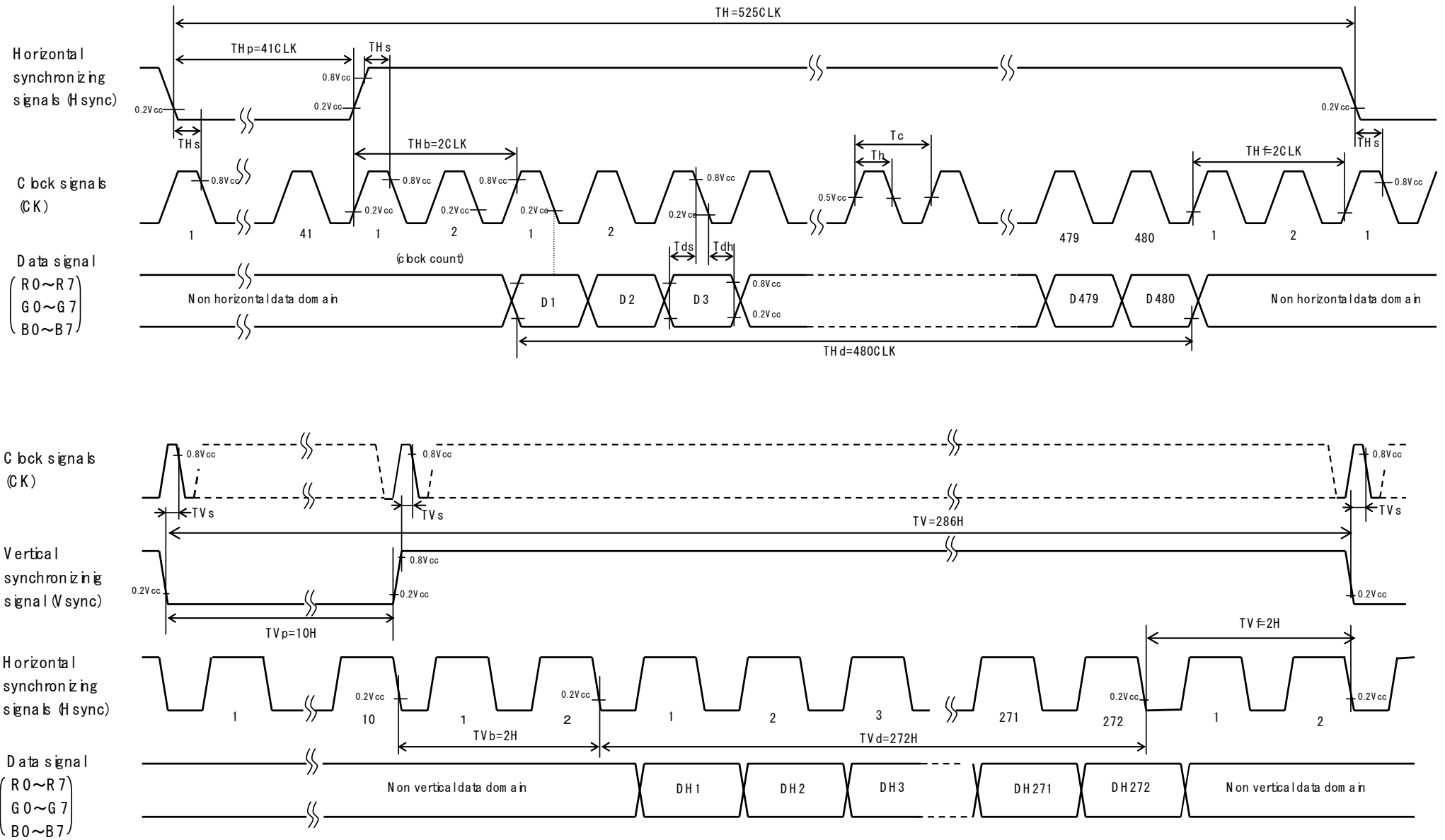
Fig 2 Input signal timing
