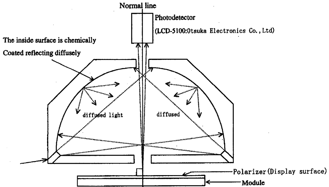
Fig. 3-2 Optical characteristics measurement method
