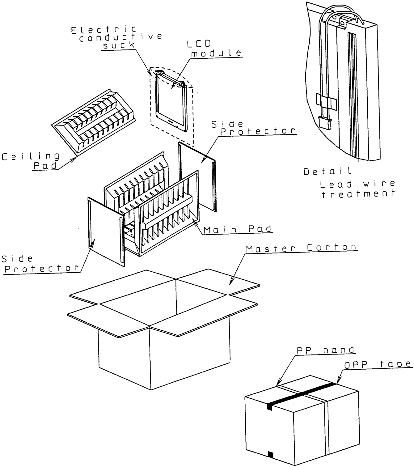
LQ121S1DG11 Packing Form
