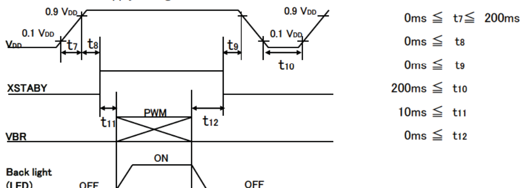
【*1】 On-off conditions for supply voltage
