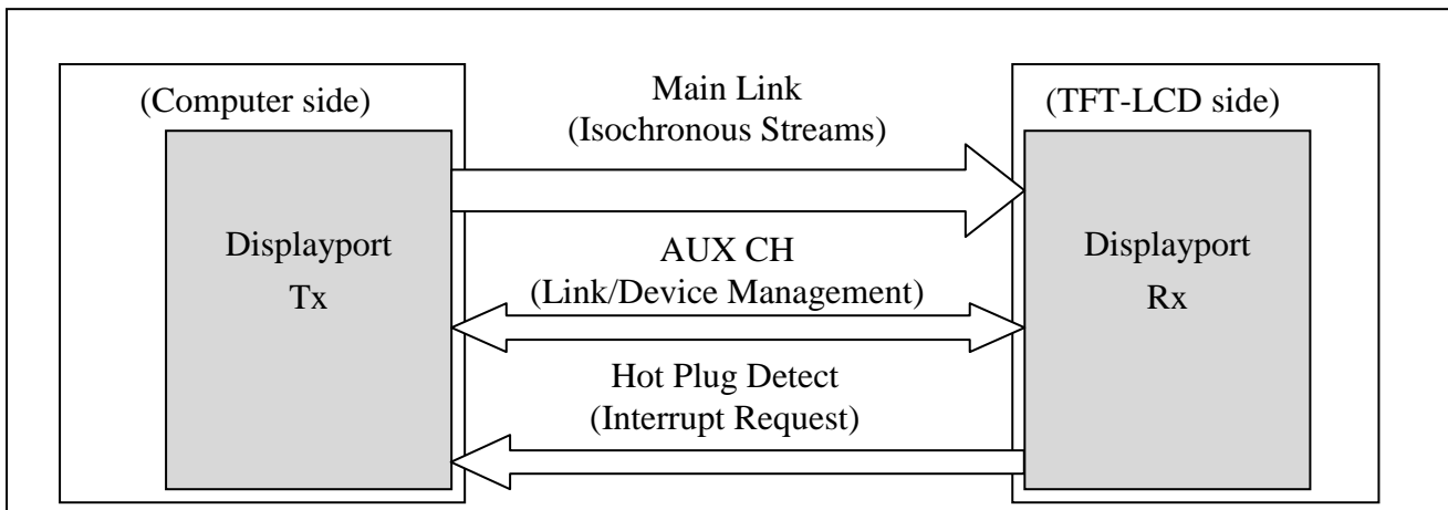
Fig.4-2-1 DP architecture.
