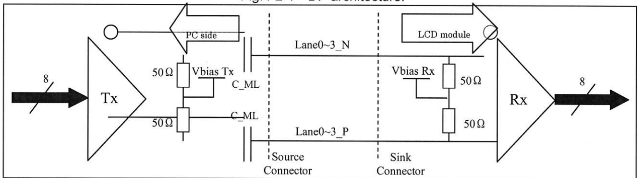
Fig.4-2-2 Main Link differential pair.
