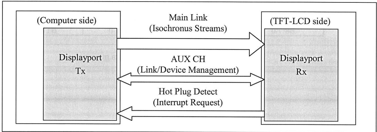
Fig.4-2-1 DP architecture.
