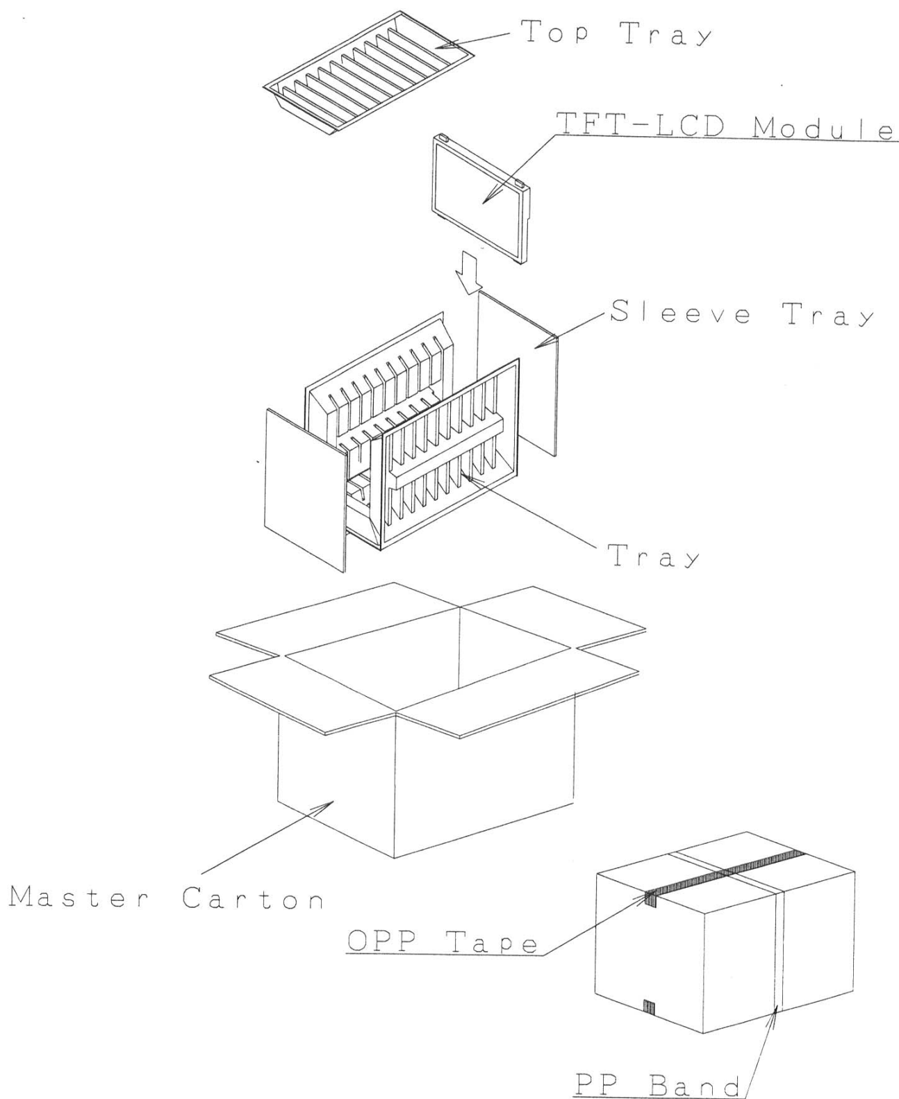
Fig3-1. Packing Form
