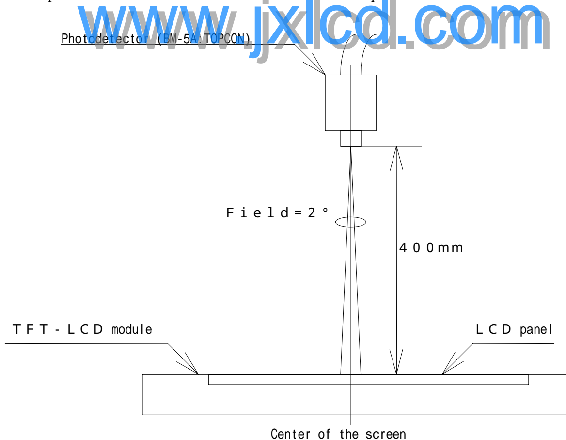
Fig.2 Optical characteristics measurement method
