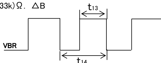
【*3】 XSTABY is connected by the pull-up(VDD) resistor of (33k)Ω. ΔB
