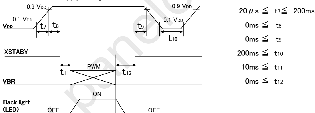
【*1】 On-off conditions for supply voltage
