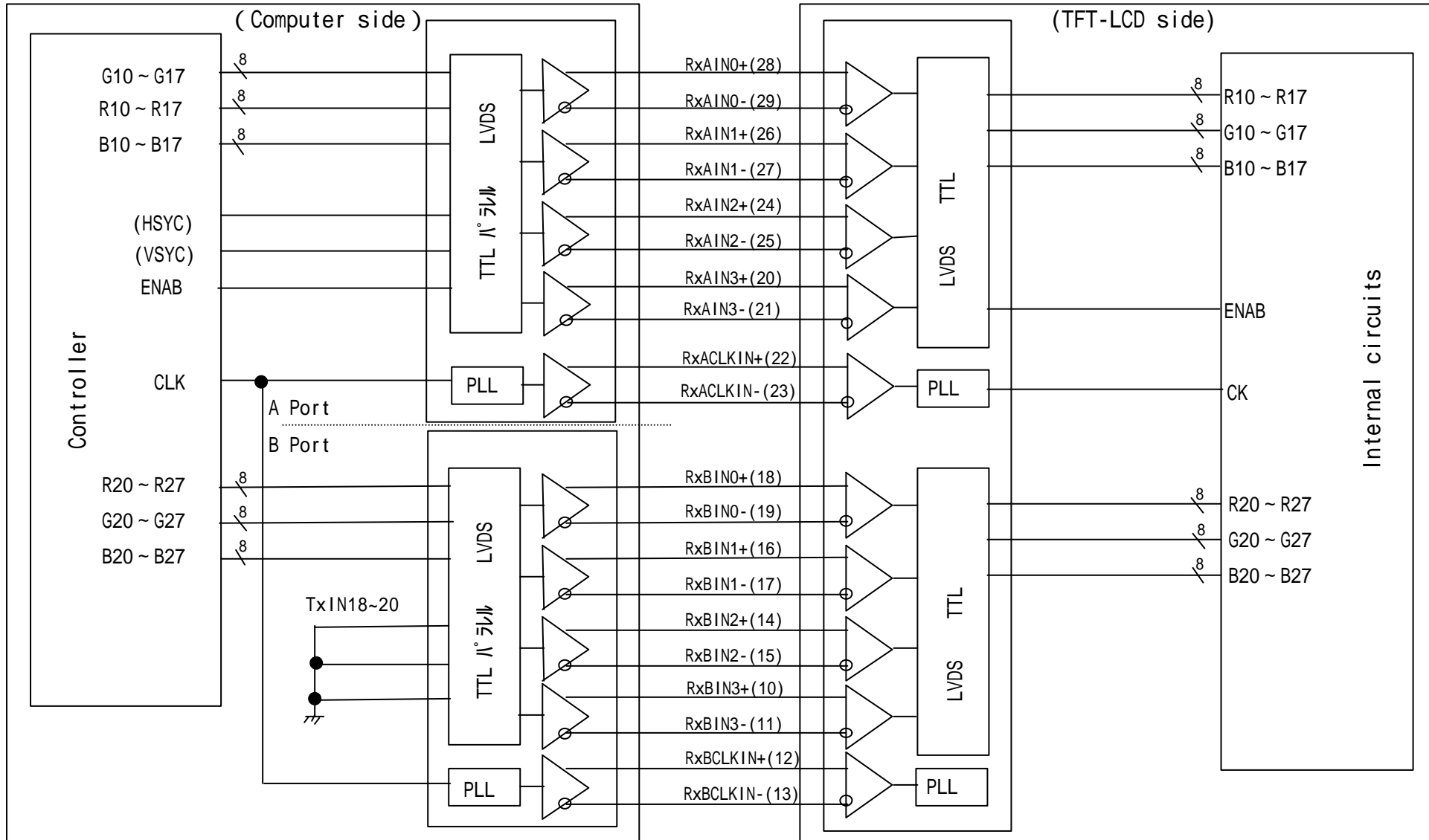
Fig.2 Interface block diagram
