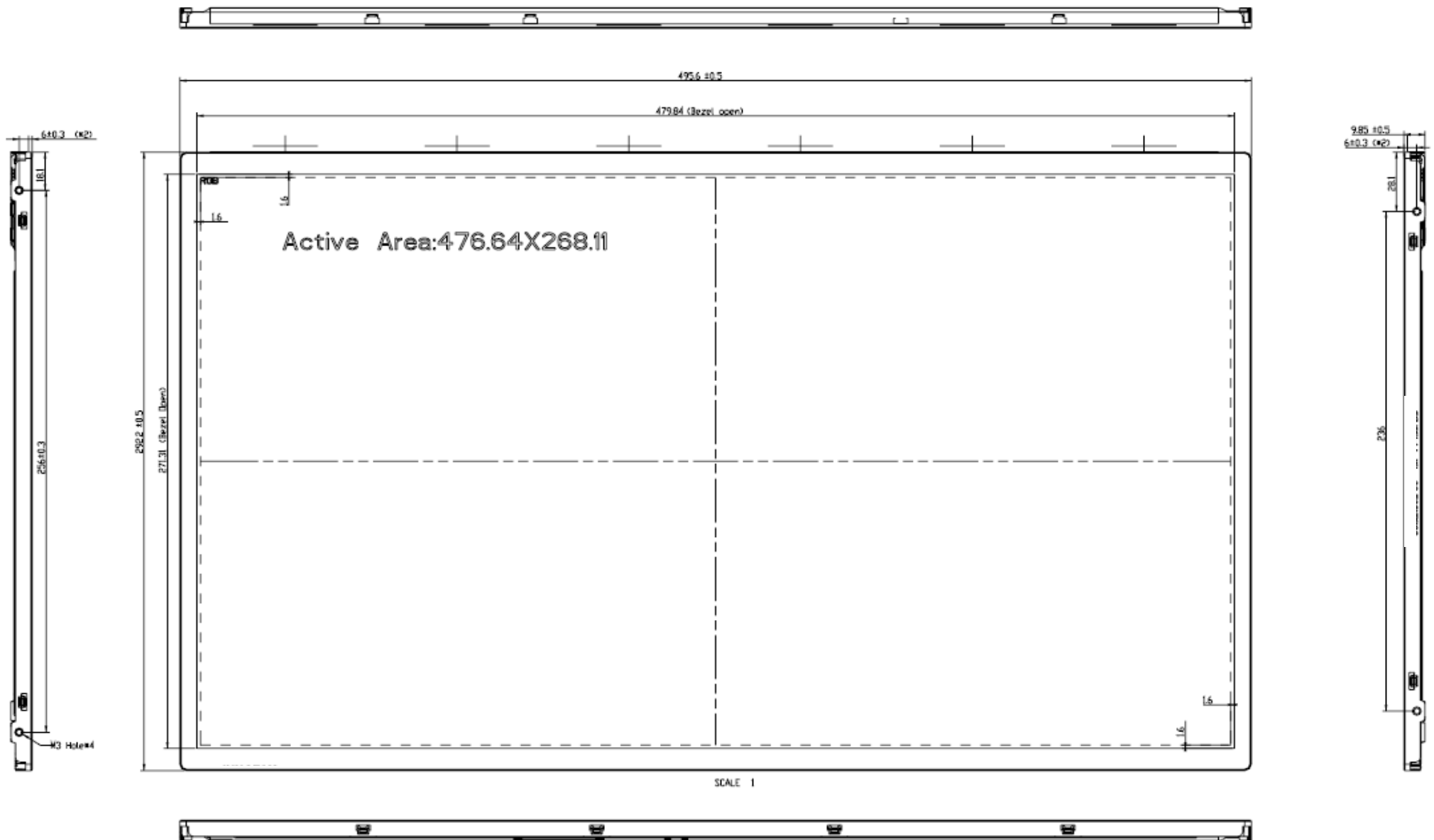
Fig. 1 Outline Dimensions Front side
